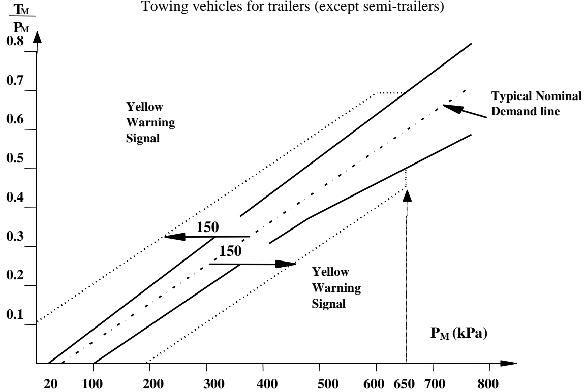
Diagram 2 Tractive units for semi-trailers
